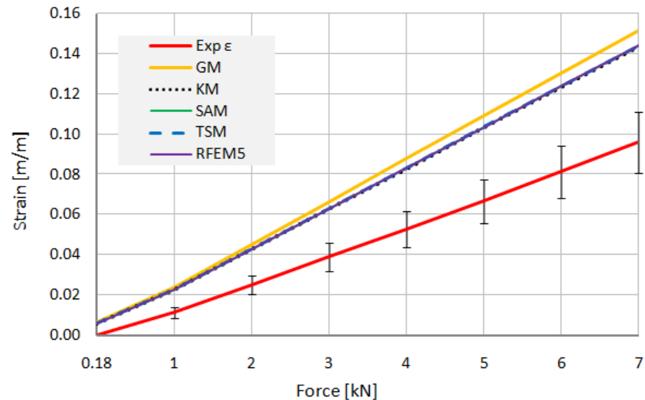
The strain in the edge fibers of outer layers as a function from the vertical load's intensity
