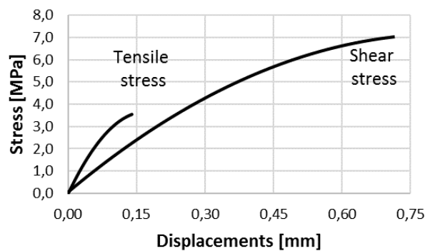
Figure 4. Stress-displacements characteristic curves of glued joints for determination of shear strength (for series with rib plywood with thickness of 6,5 mm and skin plywood with thickness of 4,0 mm with fiber direction same as applied force direction) and tensile strength (for series with rib plywood with thickness of 6,5 mm and skin plywood with thickness of 4,0 mm with fiber direction orthogonal to applied force direction).
