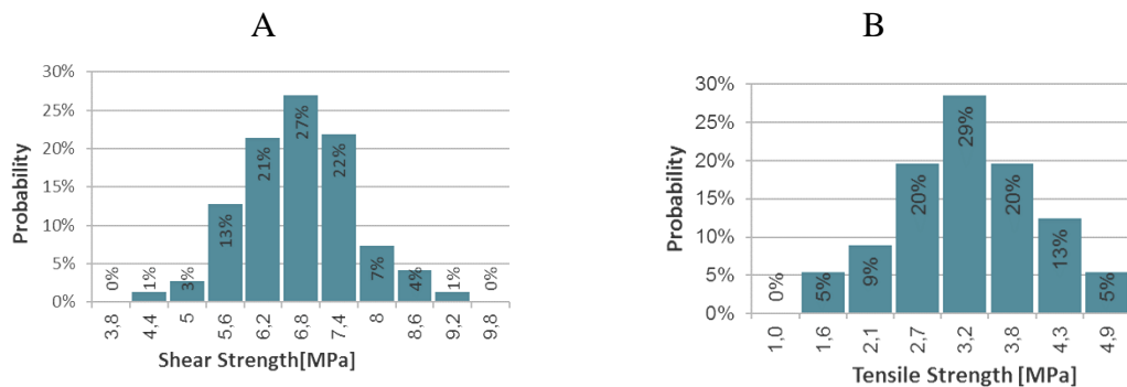
Figure 3. Histograms of plywood edge-to-surface glued joint strength: A – probability distribution of ultimate shear strength; B – probability distribution of ultimate tensile strength.
